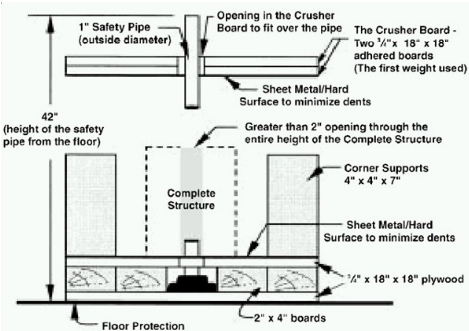
Figure B - Tester Design
